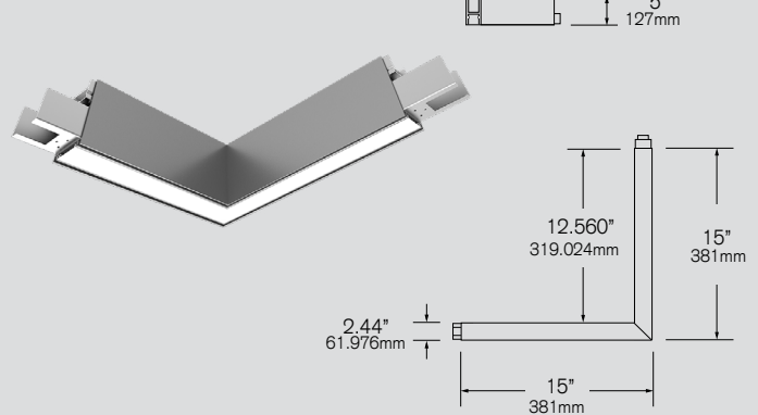
Corner
